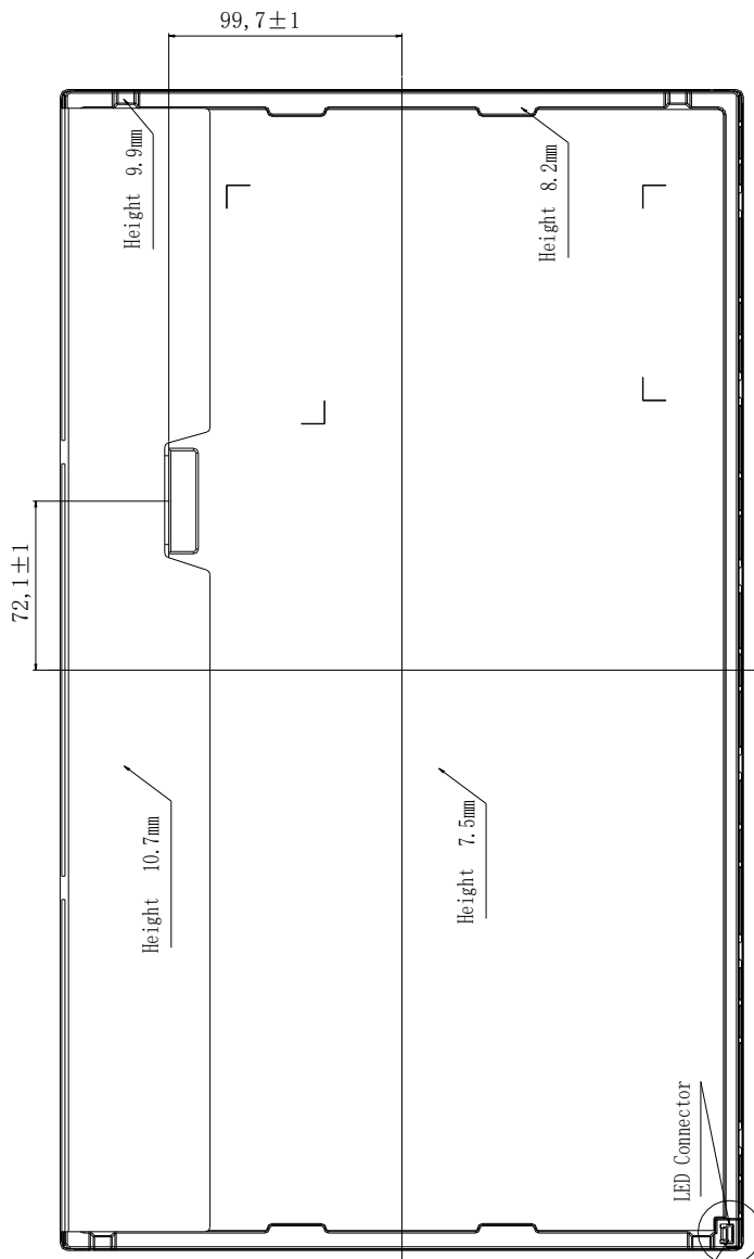
Figure 7. TFT-LCD Module Outline Dimensions (Rear view , Vertical placement)
