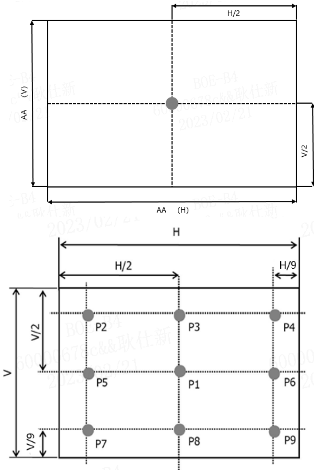
< Figure 5. White Luminance and Uniformity Measurement Locations >
