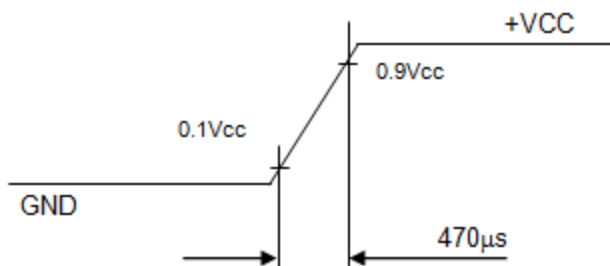
Vcc rising time is 470µs
