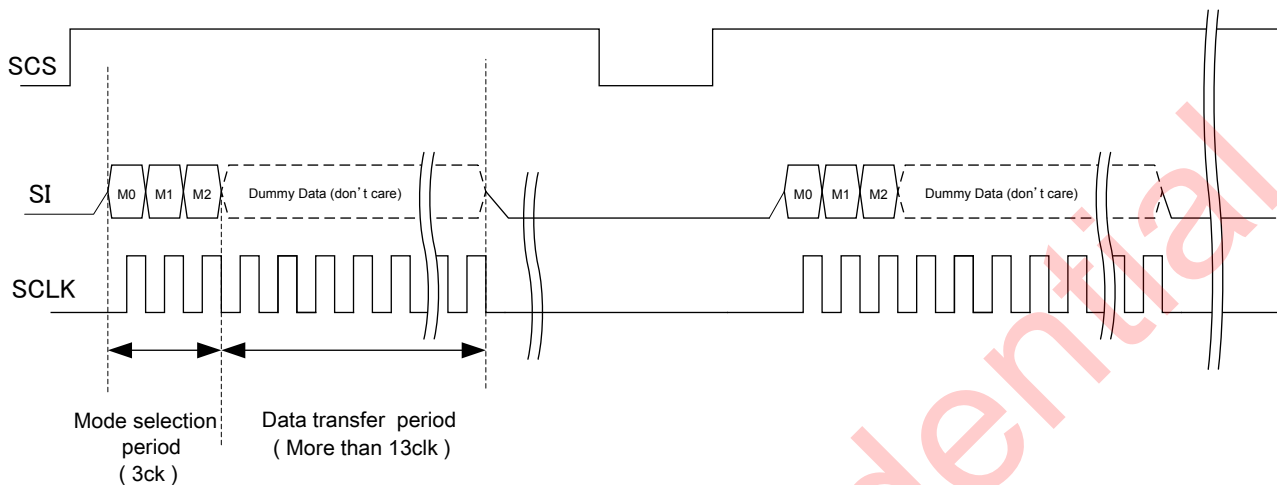
Figure 6-8 Display mode
