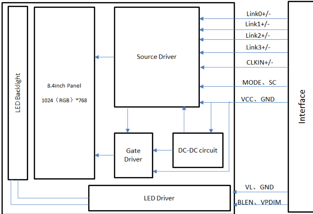
Figure 5.4.1 LCD Module Block Diagram
