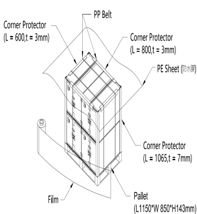
Air Transportation 單棧堆疊(2 Layers)
