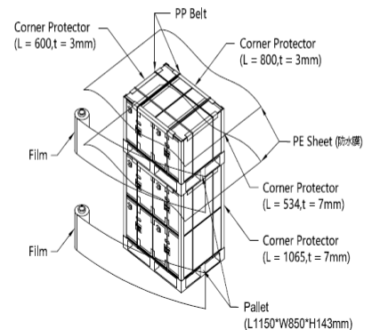
Sea / Land Transportation (40ft Container) 上,下棧堆疊(2+1 Layers)
