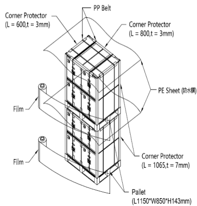
Sea / Land Transportation (40ft HQ) 上,下棧堆疊(2+2 Layers)
